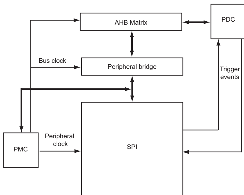
Figure 33-1. Block Diagram
