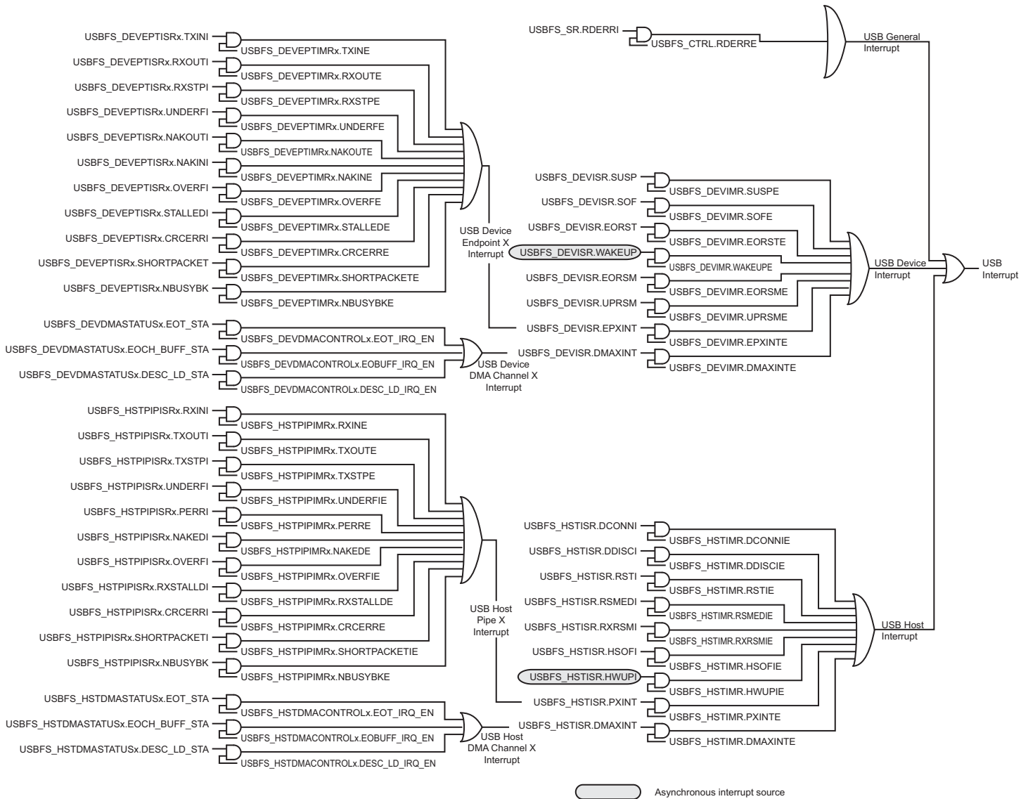
Figure 45-6. Interrupt System
