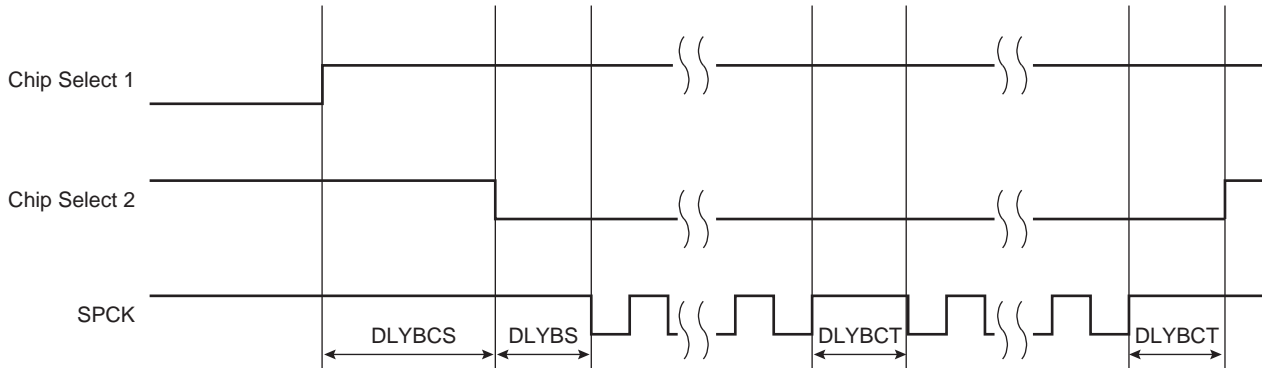
Figure 33-9. Programmable Delays
